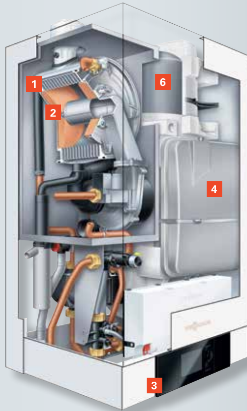
Vitodens 222-W
